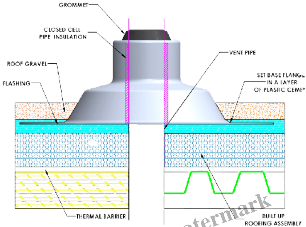
SECTION DETAIL THROUGH BUR (CONCRETE OR STEEL DECK)
