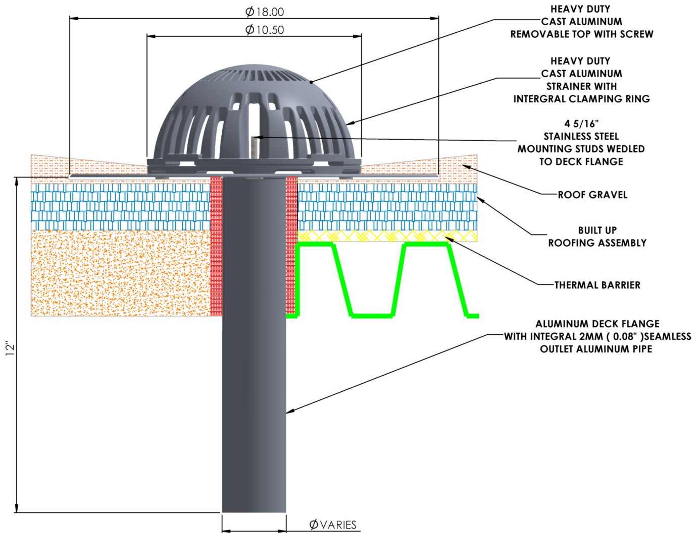
SECTION DETAIL THROUGH BUR ( CONCRETE OR STEEL DECK)
