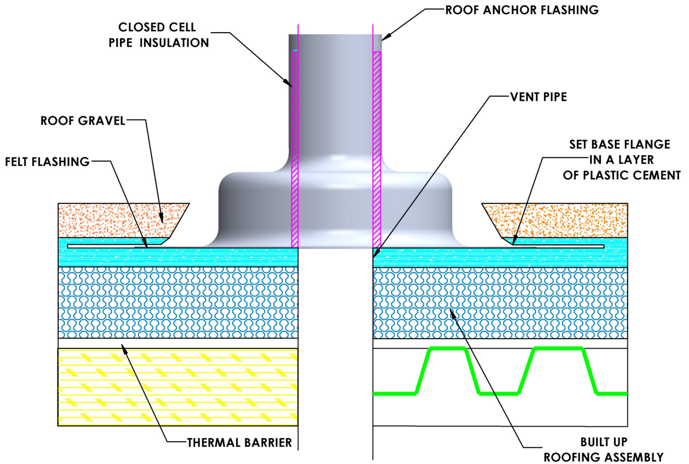
SECTION DETAIL THROUGH BUR ( CONCRETE OR STEEL DECK)
